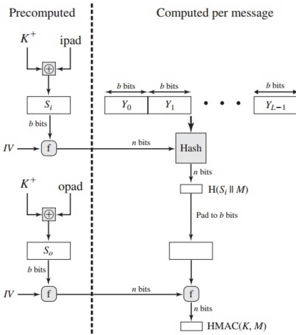
Figure 12.6 Efficient Implementation of HMAC
