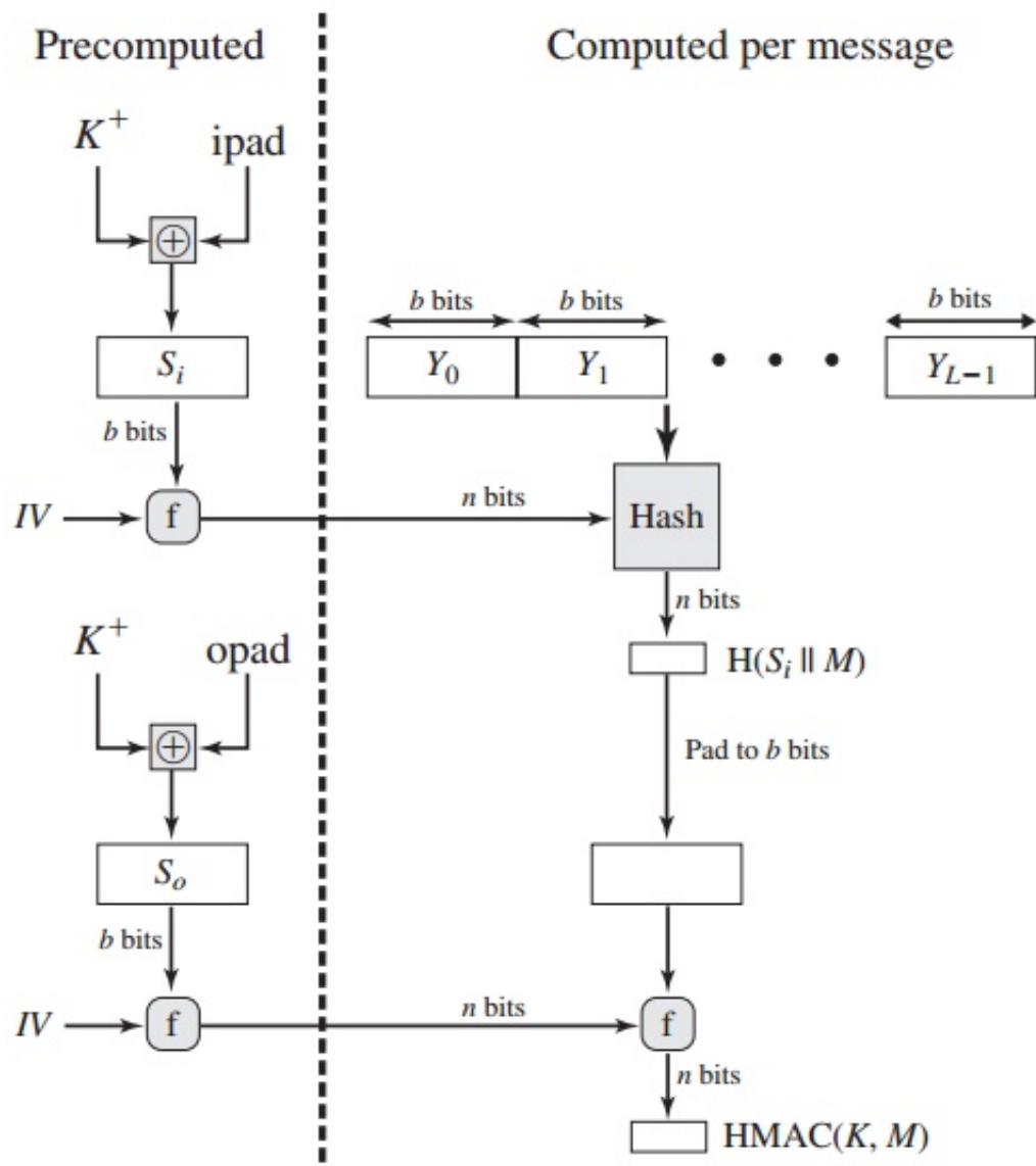
Figure 12.6 Efficient Implementation of HMAC
